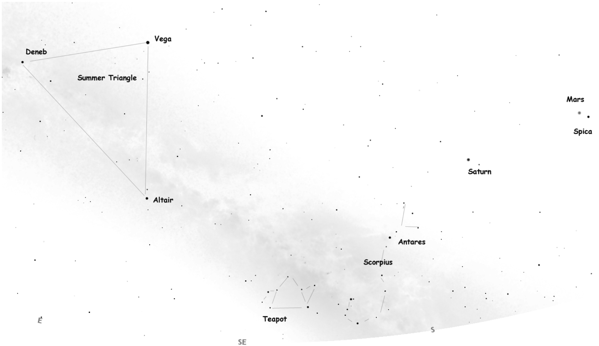
The Big picture - looking south southeast an hour after sunset in Mid-July from mid-northern latitudes.
